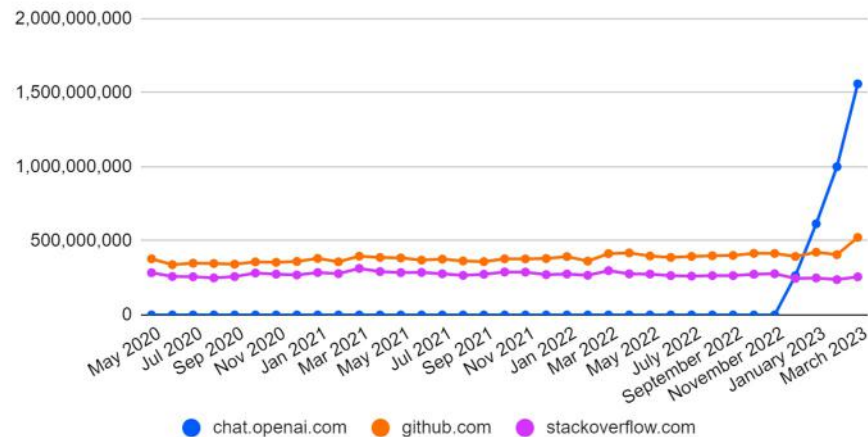
Stack Overflow vs. ChatGPT and GitHub
