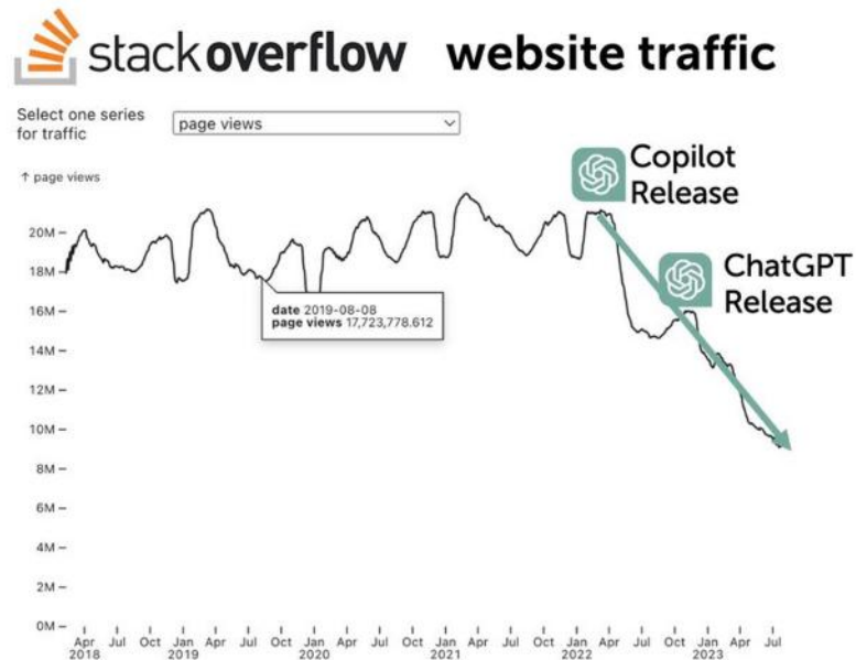
Stack Overflow vs. ChatGPT and GitHub
